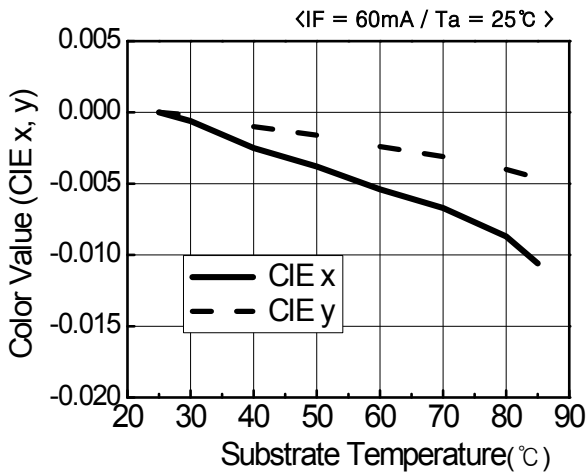
Color CIE x, y vs. Substrate Temperature
