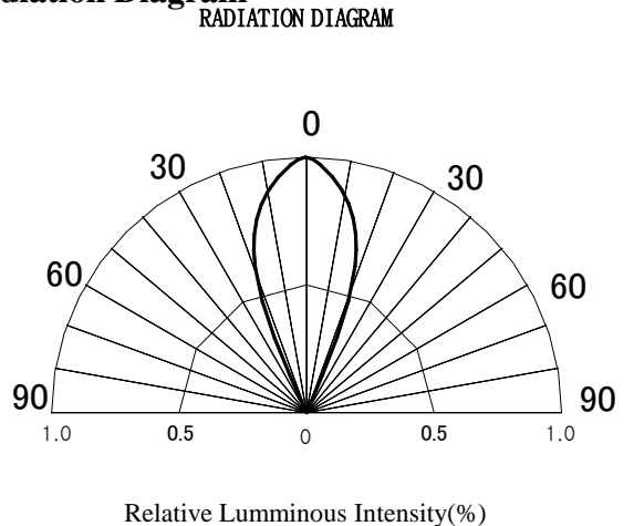
Radiation Diagram
