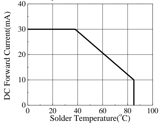
Forward Current vs. Solder Temperature
