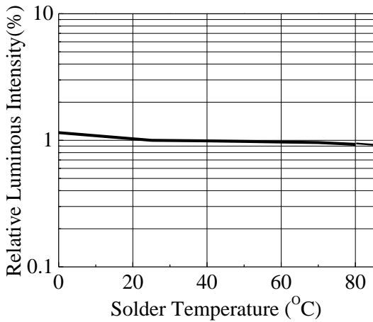
Relative Luminous Intensity vs. Solder Temperature
