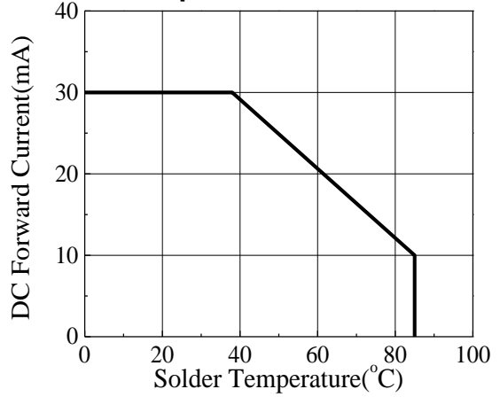
Forward Current vs. Solder Temperature
